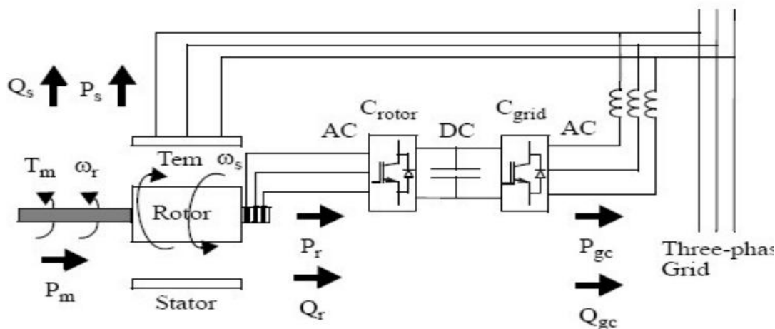
Figure 1. DFIG and its power flow.
