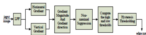
Figure 2: Block Diagram of the Canny Edge Detection
